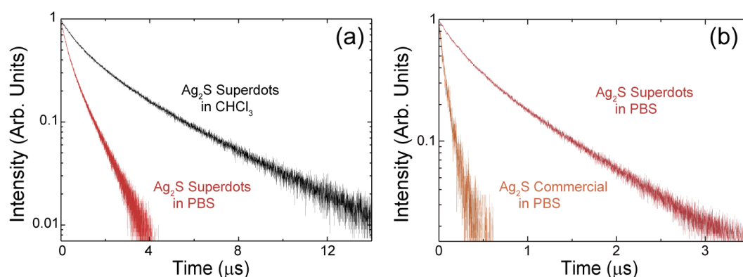
Supporting Fig. 4.15. a) Fluorescence decay curves from colloidal solutions of Ag 2 S Superdots in CHCl 3 and after transfer it to PBS through ligand exchange procedure explained above. b) Fluorescence decay curves from colloidal solutions of Ag 2 S Superdots and commercial ones. In both cases, particles are coated with PEG and dispersed in PBS.
