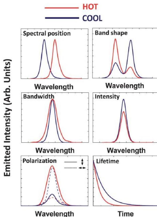
Figure 1.3: Schematic representation of the possible effects caused by a temperature increment on the luminescence. Red lines correspond to higher temperatures. This figure is reprinted with permission from Jaque, D. and F. Vetrone, Luminescence nanothermometry. Nanoscale , 2012, 4(15): p. 4301-4326.
